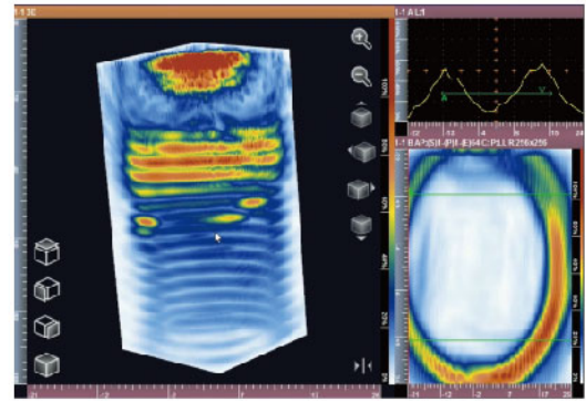
TFM 3D real-time imaging for bolt
