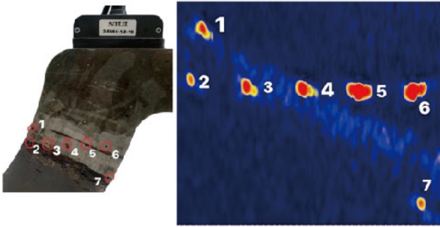
Austenitic butt weld test block
